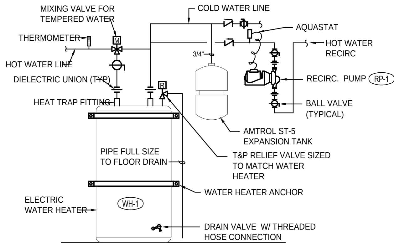
WATER HEATER PIPING DETAIL NO SCALE
